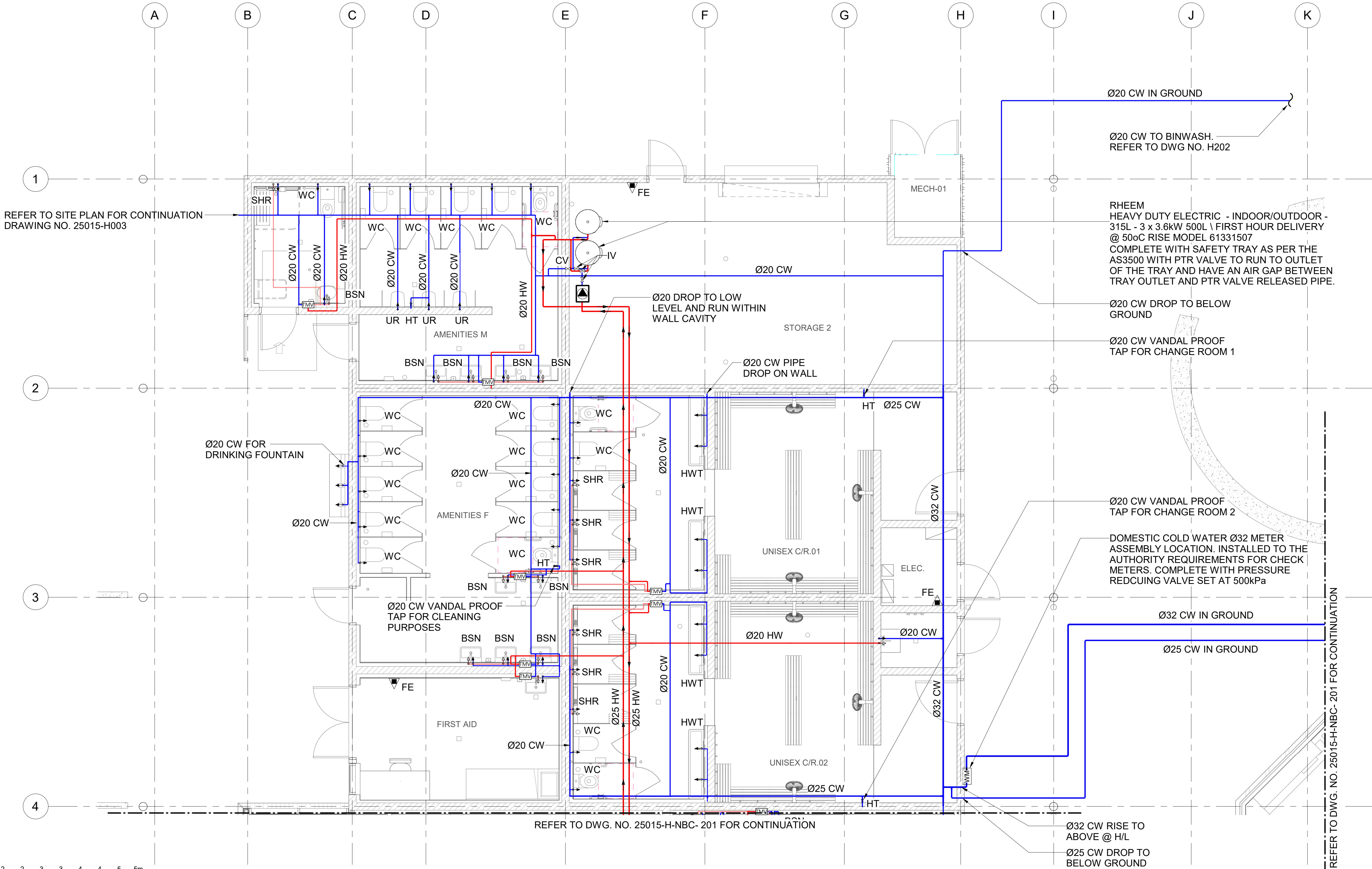
GROUND FLOOR WATER RETICULATION LAYOUT - PART PLAN 1
